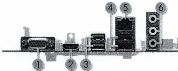
Figure : Lubin back I/O panel
